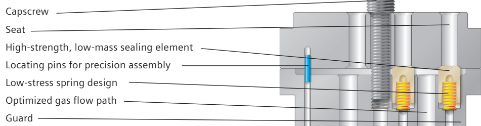
Cross Section of Magnum Valve
