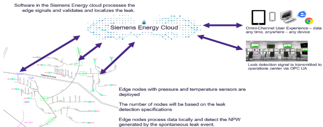
Figure 2. Siemens Energy SLD Service Architecture, powered by ProFlex Technologies
