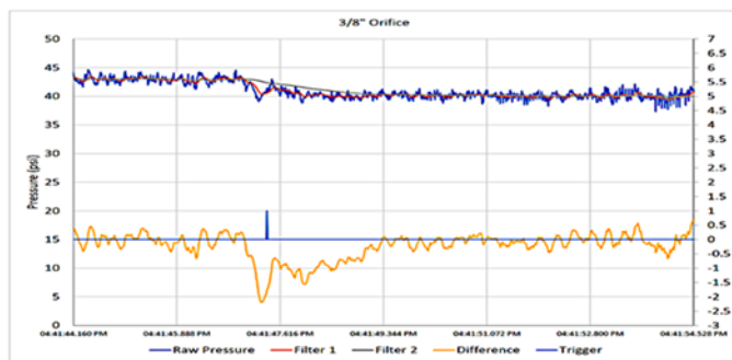
Figure 1. Enhanced negative pressure wave detection identifies leaks within seconds.
