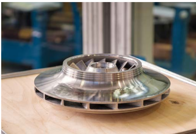
Figure 1. Additively manufactured radial impeller after overspeed test.
