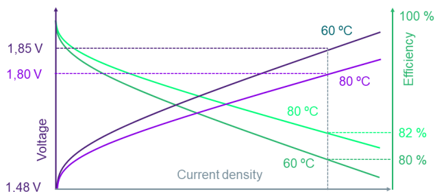
Figure 5: Schematic showing the effect of temperature on efficiency
