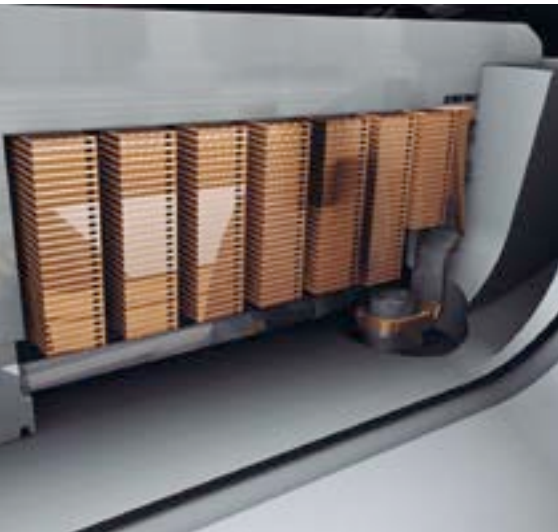
Fig. 2: Inner-cooled winding design
