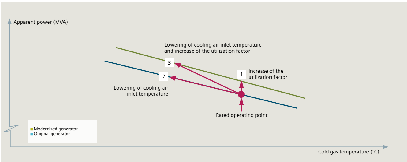
Fig. 4: Uprate as a function of cold gas temperature
