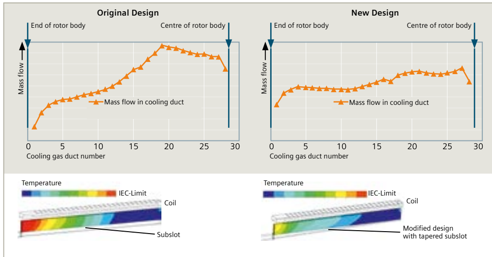
Fig. 3: Homogeneous cooling air flow, particularly at rotor ends and reduced temperatures based on modified subslot design (at right) versus original design (at left)
