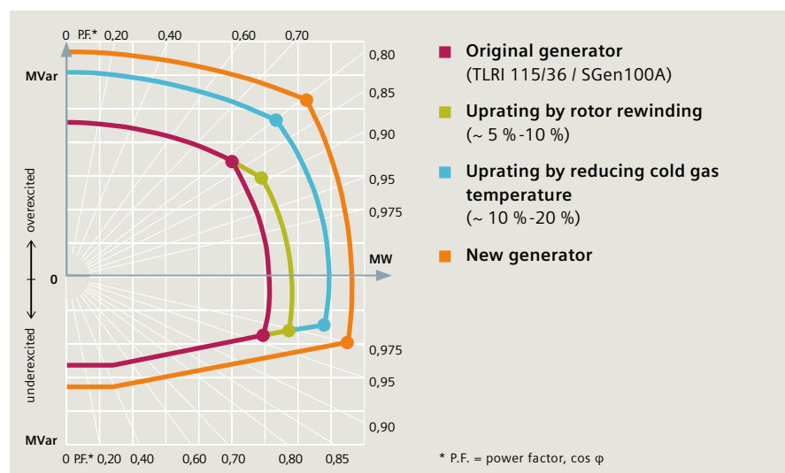
Fig. 1: Schematic showing various uprating options based on performance curves
